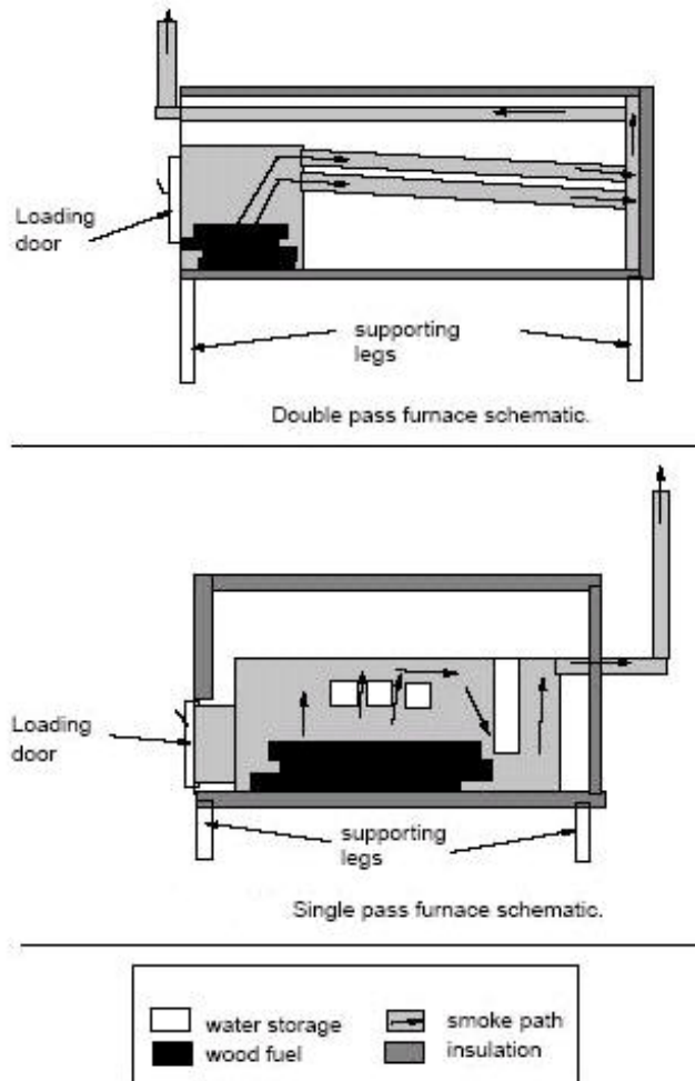
Figure 2: Schematic of Inside OWB 4
