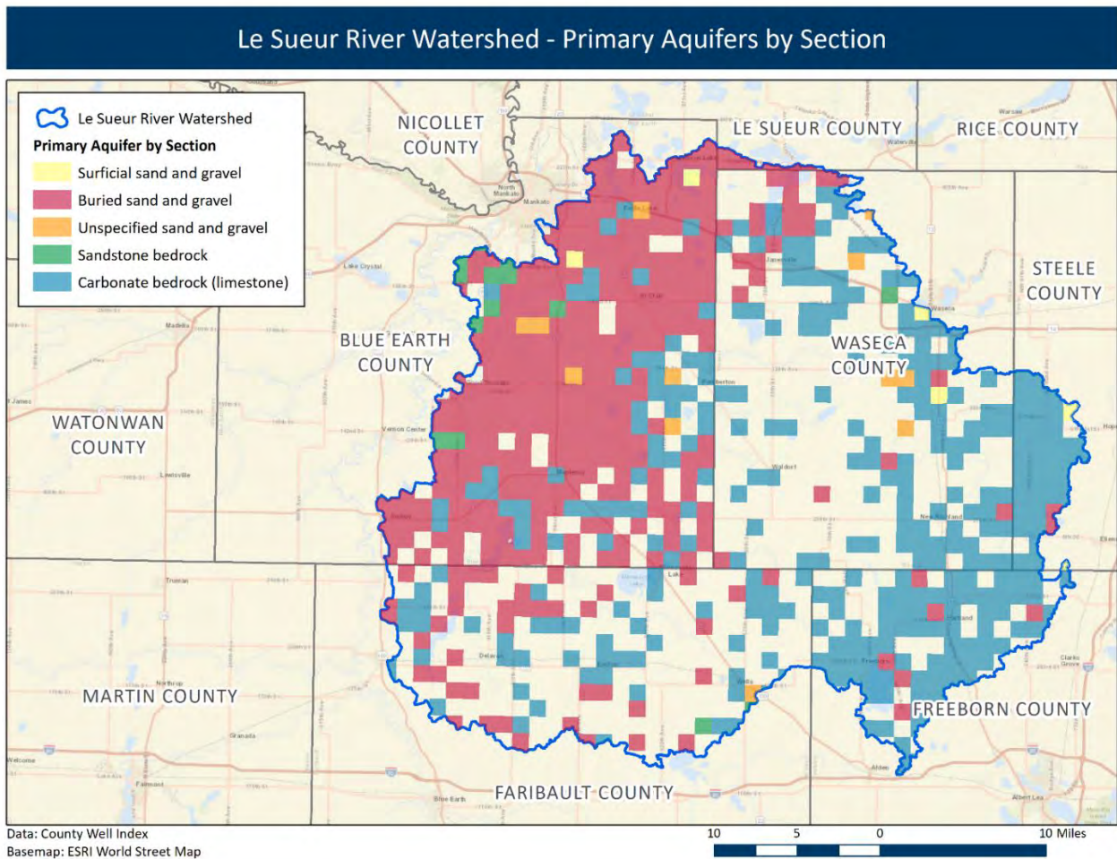
Figure 4: Le Sueur River Watershed – Primary Aquifers by Section. Buried sand and gravel aquifers are the primary drinking water source for Blue Earth County, with carbonate bedrock as the primary source for the rest of the watershed. Completed County Geologic Atlases will further inform this dataset. Blue Earth County has the only completed County Geologic Atlas for the watershed.
