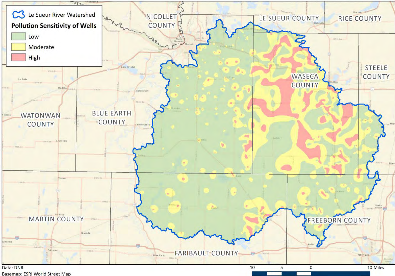
Figure 7: Le Sueur River Watershed - Pollution Sensitivity of Wells.
