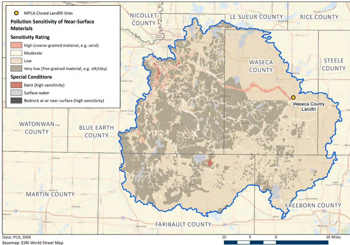
Figure 20: Le Sueur River Watershed - MPCA Closed Landfill
