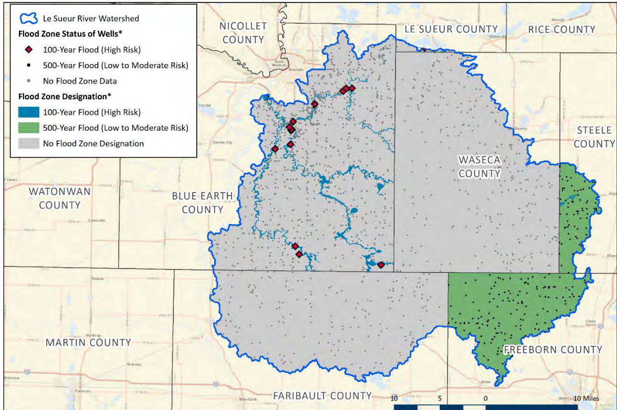
Figure 13: Le Sueur River Watershed – Drinking water wells and flood zone risk to contamination.
