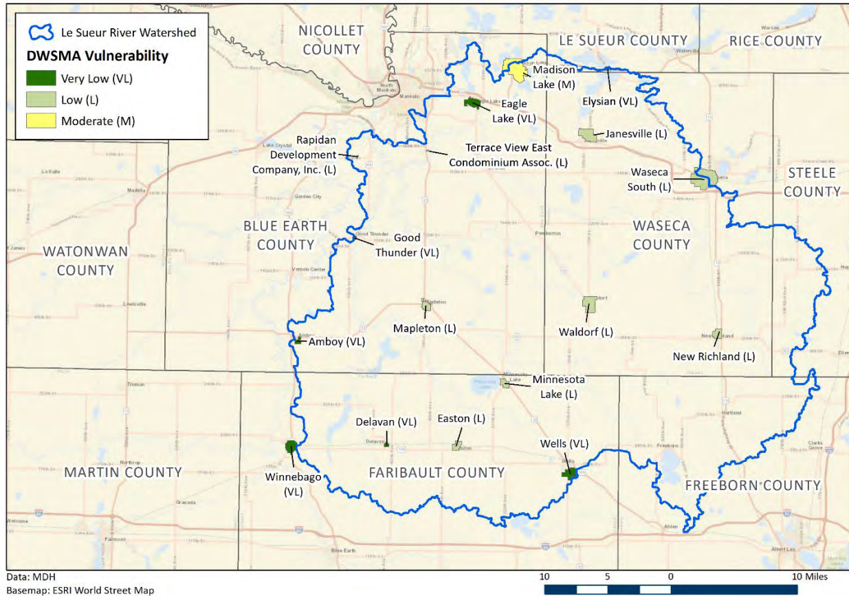
Figure 10: Le Sueur River Watershed - Drinking Water Supply Management Areas. There are 17 approved Drinking Water Supply Areas (DWSMA) for community public water supply systems in the watershed.
