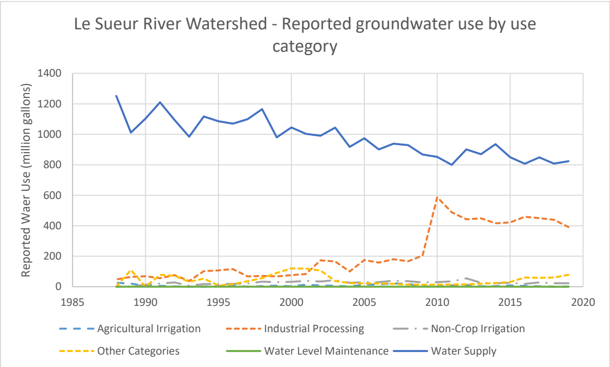
Figure 23: Reported groundwater use from DNR permit holders by use category. Most permitted groundwater withdrawals are used for water supply. Pumping for water supply declined from approximately 1200 million gallons per year in 1988 to approximately 800 million gallons per year in 2016, and then stayed fairly level. Industrial processing increased from 200 to 600 million gallons per year in 2010.
