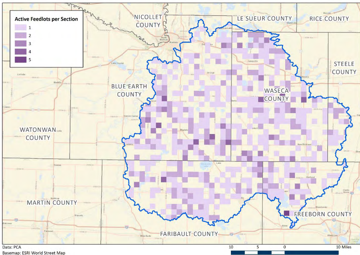
Figure 18: Le Sueur River Watershed – Active Feedlots. There are 787 active feedlots within the watershed.
