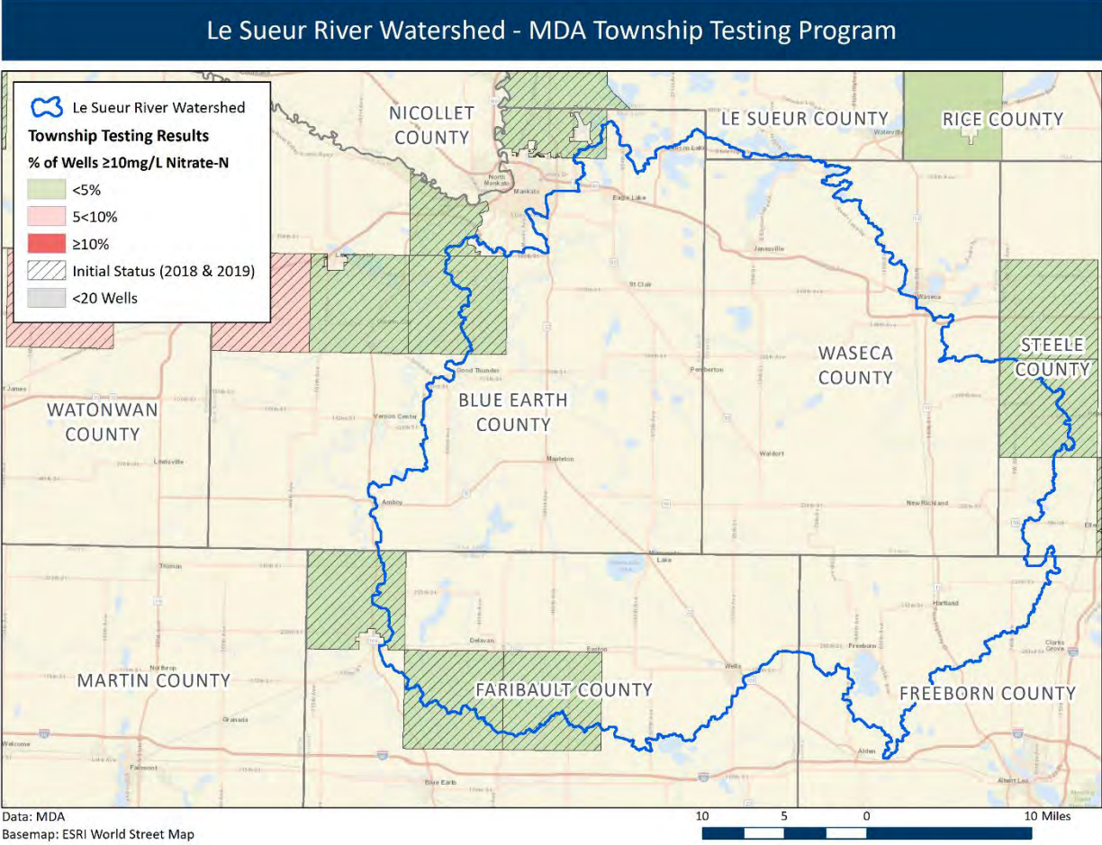
Figure 15: Le Sueur River Watershed – MDA Township Testing Program ‘Initial’ results.
