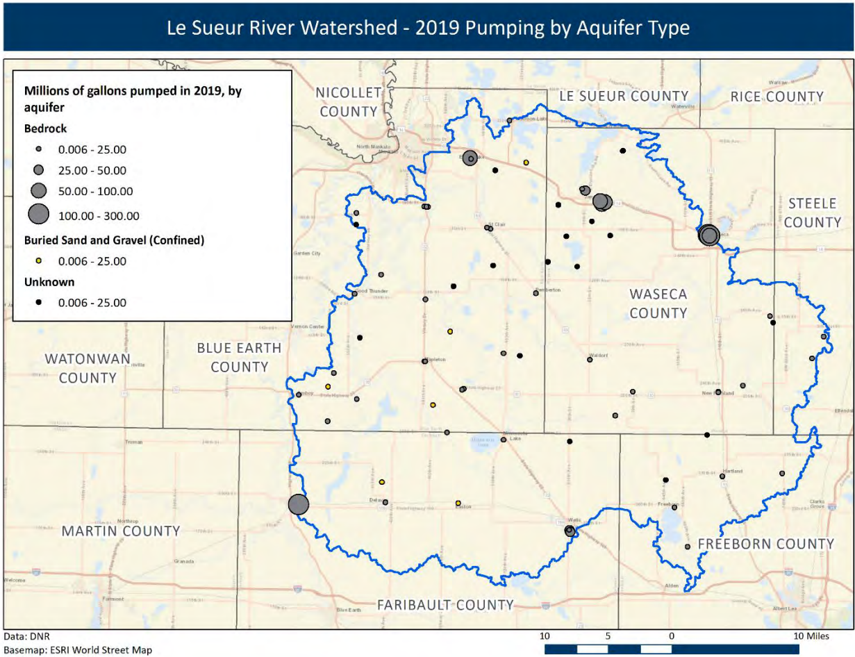
Figure 25: Le Sueur River Watershed – Distribution of groundwater appropriation permits for 2019 by volume reported and aquifer category. Bedrock aquifers supply 96 percent of the reported water use.
