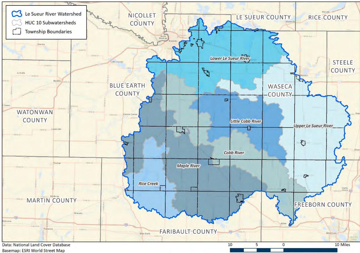
Figure 2: Le Sueur River Watershed - is comprised of six subwatersheds (HUC-10)
