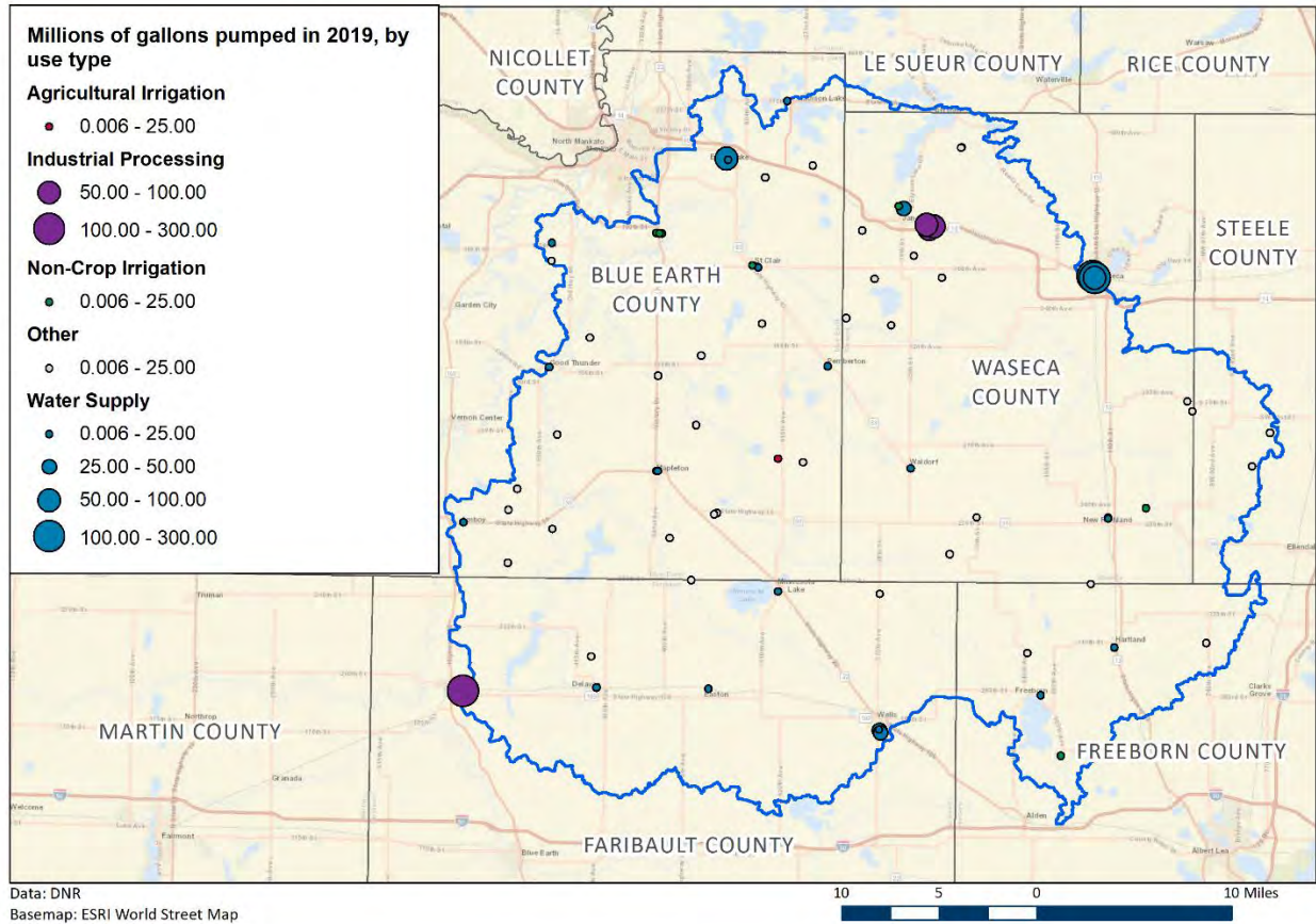
Figure 24: Le Sueur River Watershed - Distribution of groundwater appropriation permits for 2019 by volume reported and use category. The largest water users in the watershed are the cities of Waseca, Eagle Lake, and Wells and two ethanol plants. All the wells with use category other are used for livestock watering.
