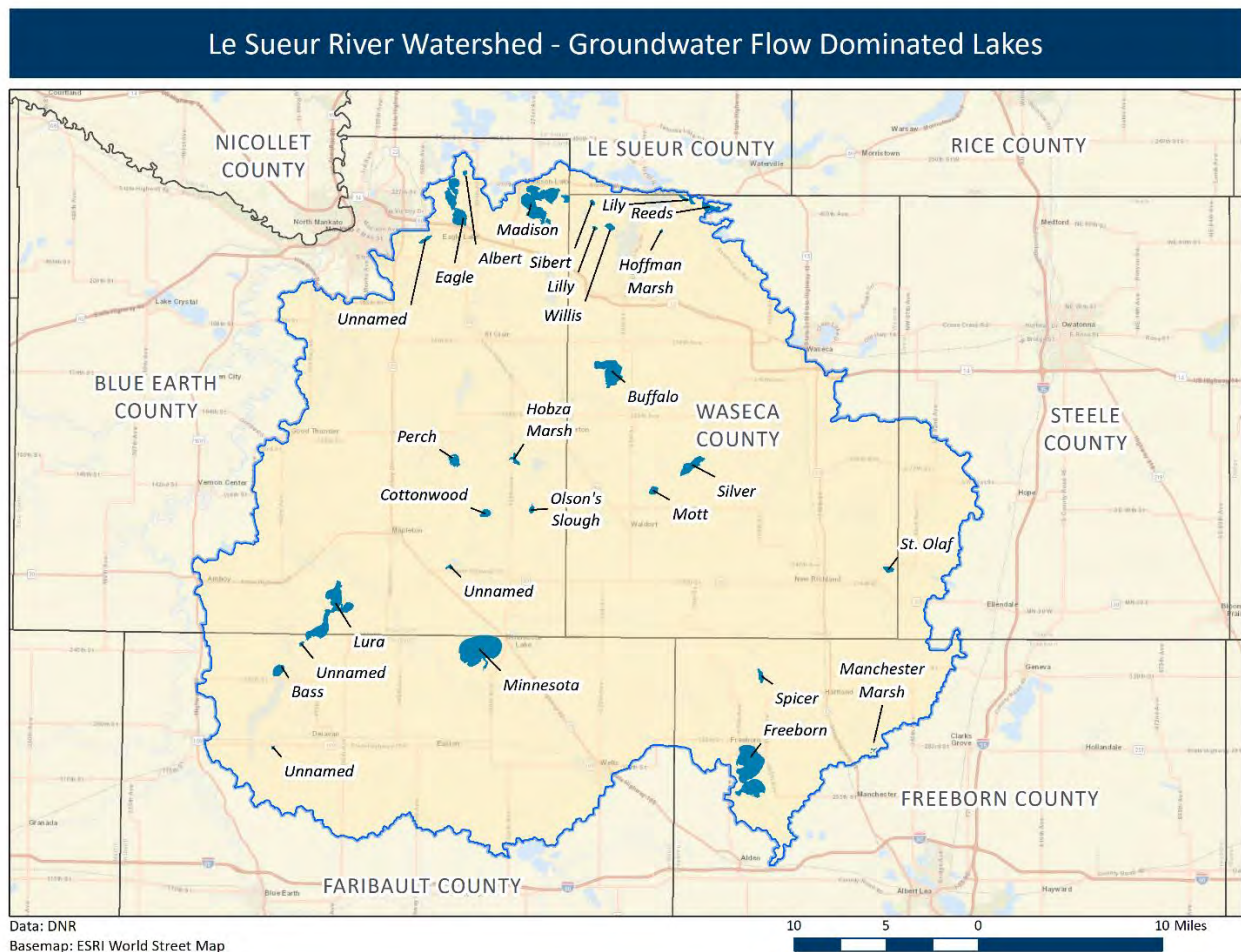
Figure 31: Groundwater-Dominated Lakes in the Le Sueur River Watershed. There are 28 groundwater-flow dominated lakes in the planning area. Of these lakes, 13 have a watershed area to lake area ratio less than 5 and are likely groundwater dominated and 15 have a watershed area to lake area ratio between 5 and 10 and may be groundwater dominated. Lake specific data should be collected before making a final determination on the amount of influence groundwater has on a particular lake.
