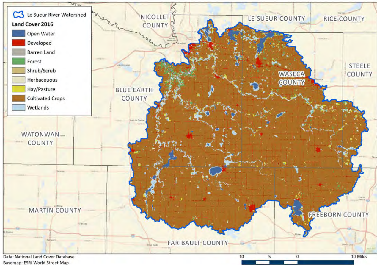
Figure 3: Le Sueur River Watershed - Land Cover. Row-crop agriculture is the predominant land cover in the watershed.
