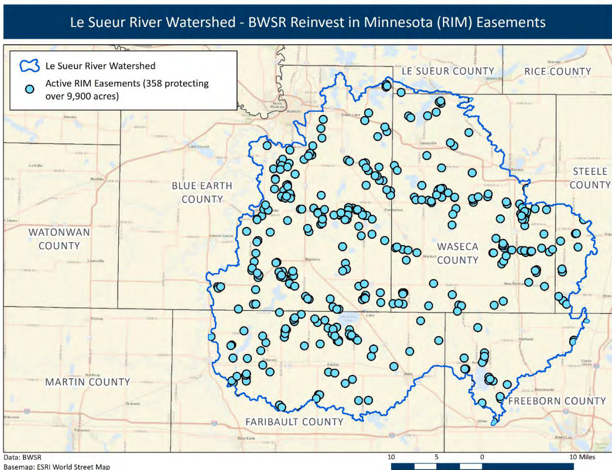
Figure 33: Le Sueur River Watershed – BWSR RIM easements
