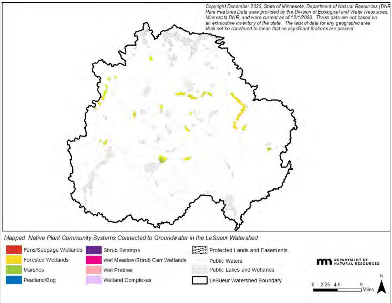
Figure 29: Le Sueur River Watershed – Native Plant Communities Connected with Groundwater
