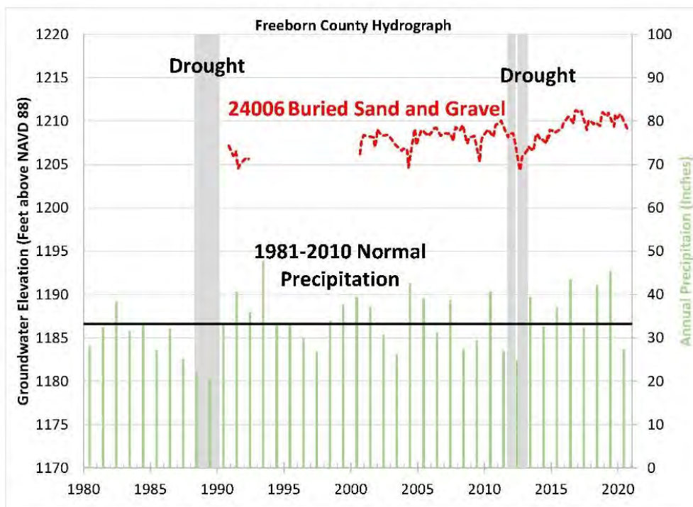
Figure 28: Hydrographs of well 24006 compared to precipitation. The water level in the buried sand and gravel aquifer has been rising since the start of the continuous record in 2000.
