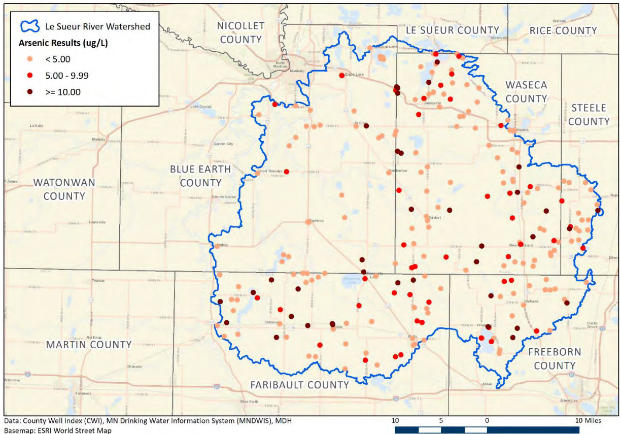
Figure 16: Le Sueur River Watershed - Arsenic Results
