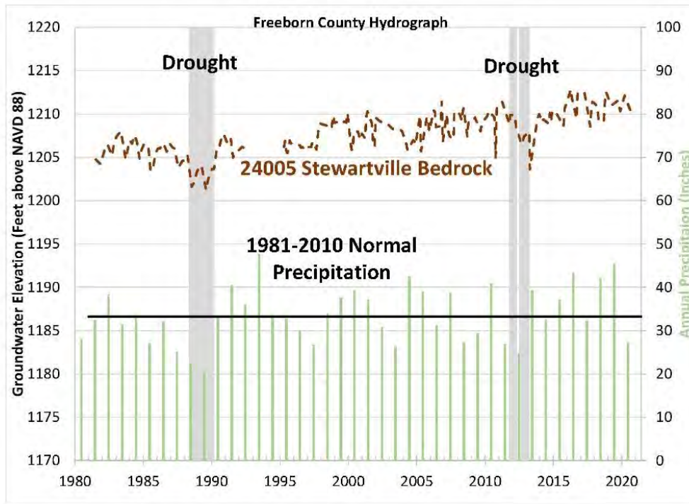
Figure 27: Hydrograph of well 24005 compared to precipitation. The water level in the Stewartville aquifer has been rising since 1990 due to many wet years with higher than normal precipitation.
