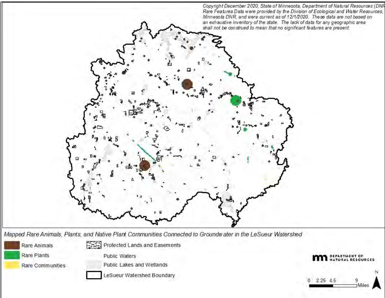
Figure 30: Le Sueur River Watershed - Rare Plants, Animals, and Native Plant Communities Connected with Groundwater
