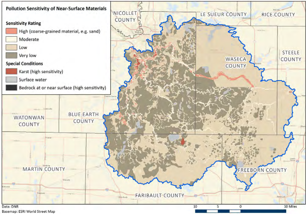
Figure 5: Le Sueur River Watershed - Pollution Sensitivity of Near Surface Materials
