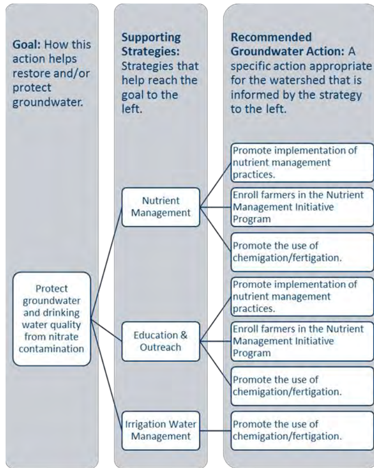
Figure 32: Visual representation of the relationship between goals, supporting strategies, and recommended groundwater action.
