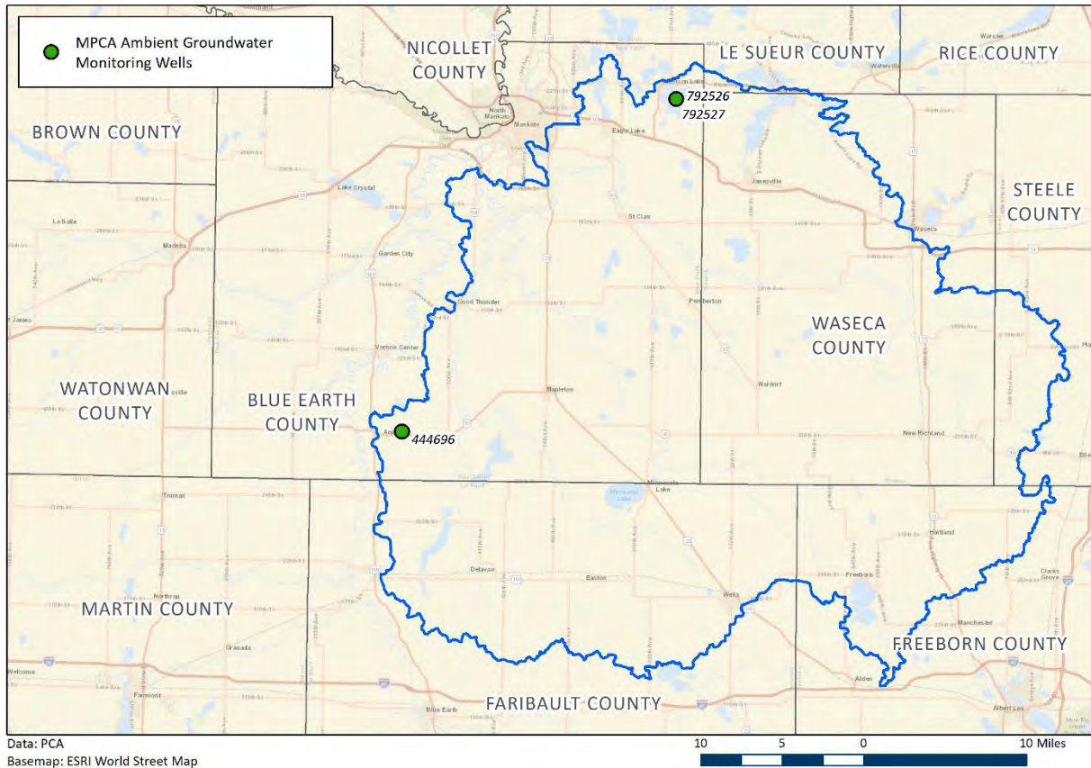
Figure 17: Le Sueur River Watershed – MPCA Ambient Groundwater Monitoring Well Network
