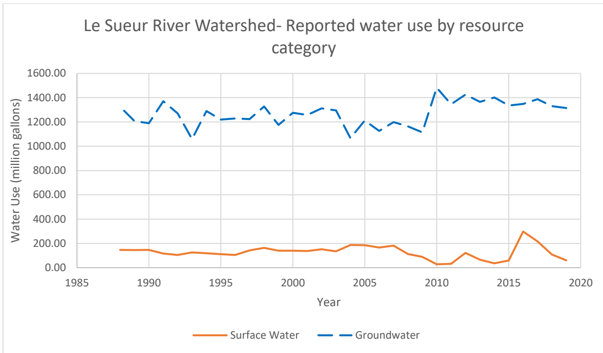
Figure 21: Reported water use from the DNR permit holders by resource category. Groundwater use increased from about 1200 million gallons per year in 1998 to about 1400 million gallons per year in 2010 and then gently declined slightly.
