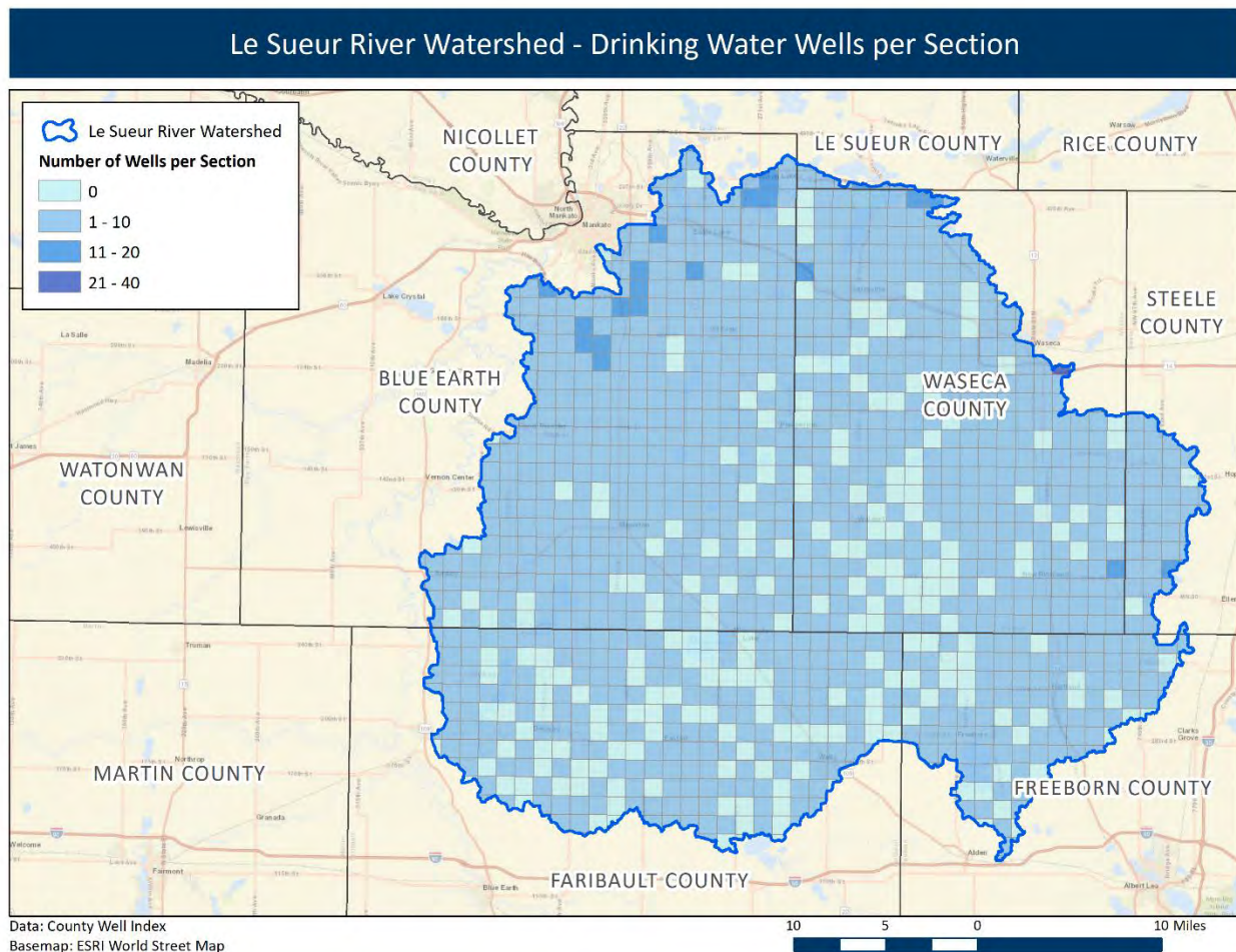
Figure 12: Le Sueur River Watershed - Density of drinking water wells per section. There are 2,270 private wells identified.
