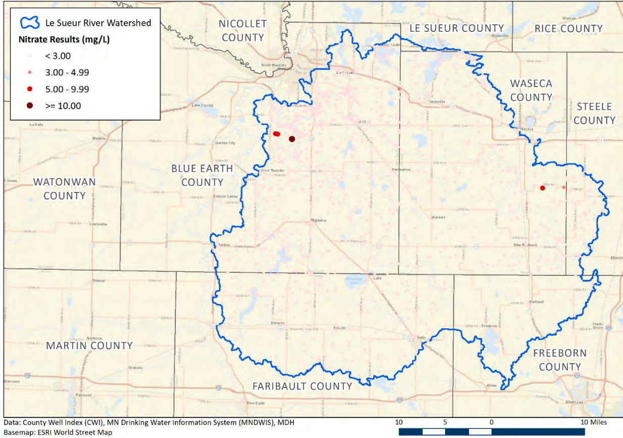
Figure 14: Le Sueur River Watershed - Nitrate results from drinking water wells.
