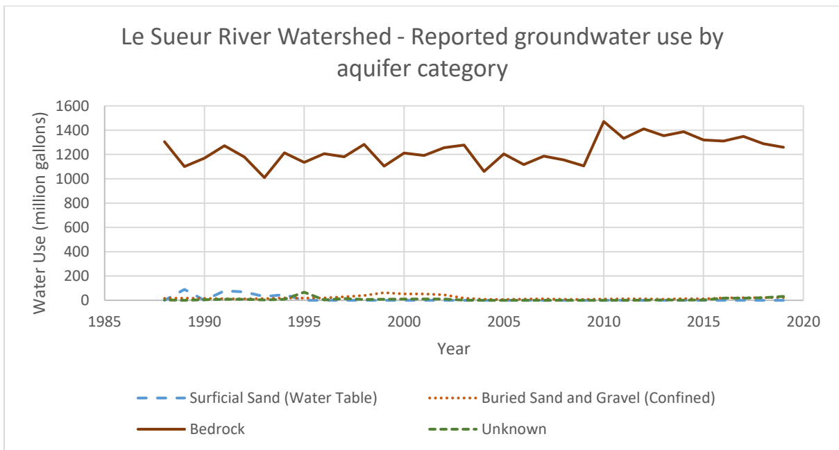
Figure 22: Reported groundwater use from DNR permit holders by aquifer category. Most permitted groundwater use is drawn from bedrock aquifers. Pumping from bedrock aquifers varied from about 1000 million gallons per year to 1400 million gallons per year.
