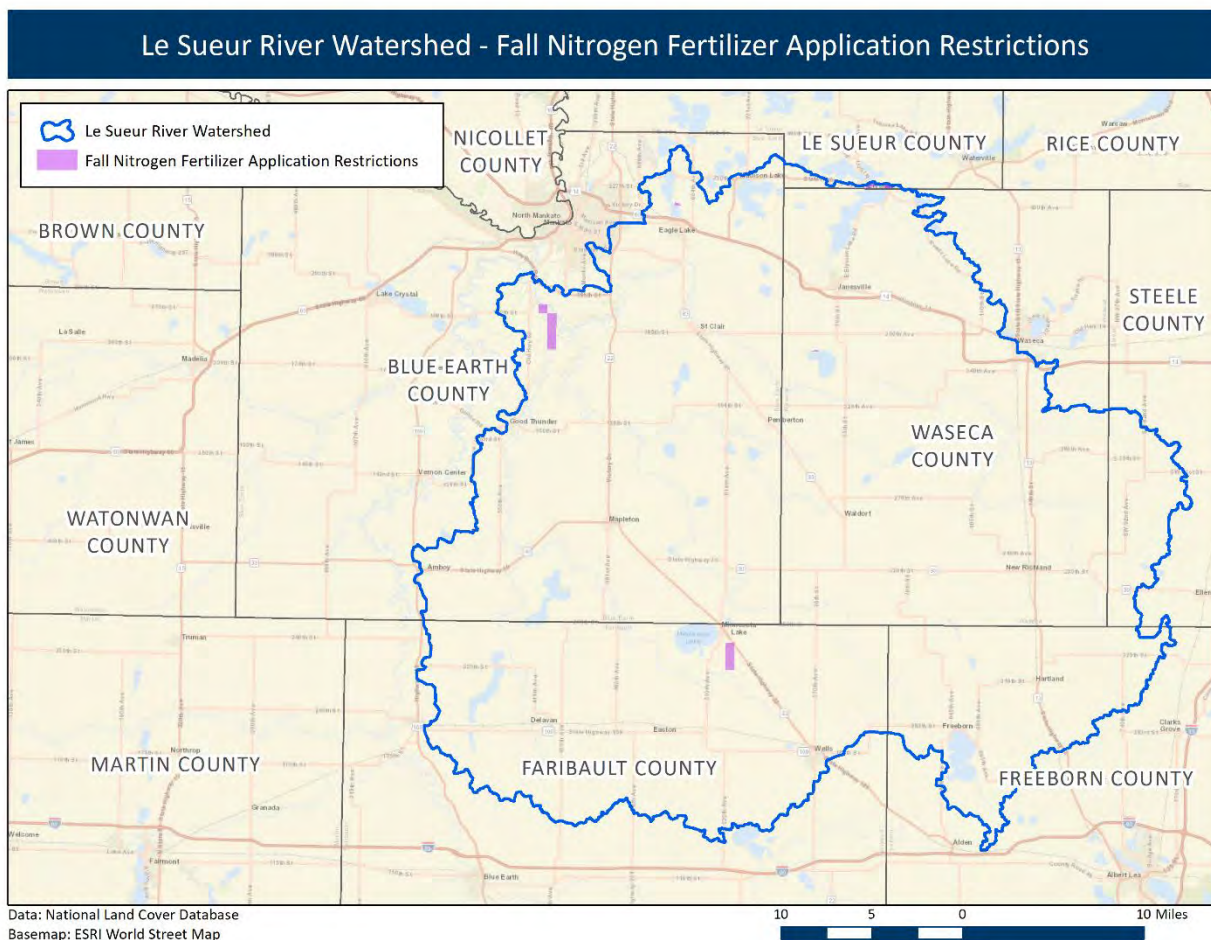
Figure 11: Le Sueur River Watershed – MDA Fall Nitrogen Fertilizer Restrictions
