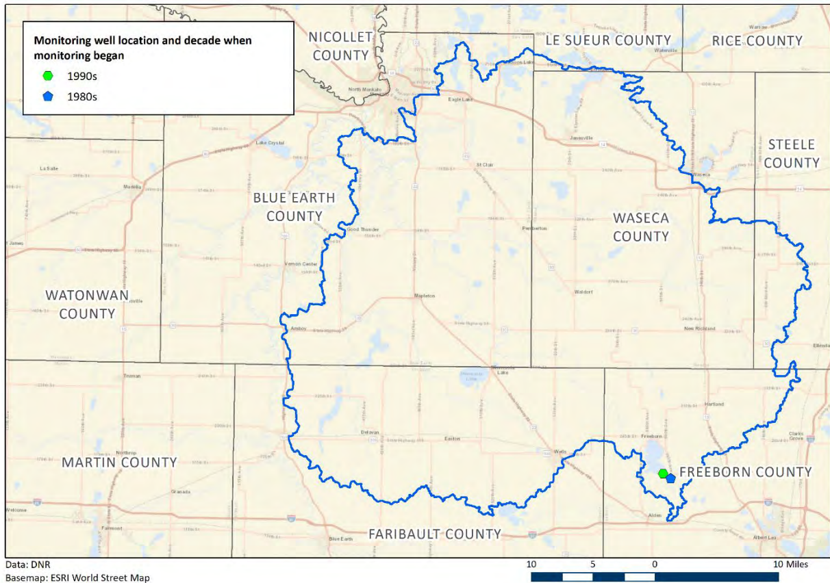
Figure 26: Le Sueur River Watershed – Active Groundwater-Level Monitoring Wells by decade monitoring started. Two wells are measured for groundwater levels in the watershed. One of the groundwater-level monitoring wells in the watershed has been monitored since the 1980s and one since the 1990s. Both wells have hydrographs.
