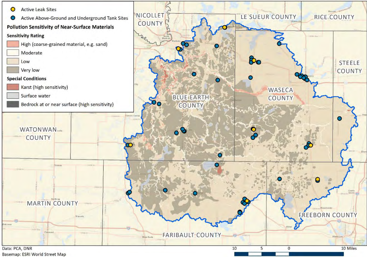
Figure 19: Le Sueur River Watershed - MPCA Active Tank and Leak Sites and Pollution Sensitivity of Near-Surface Materials
