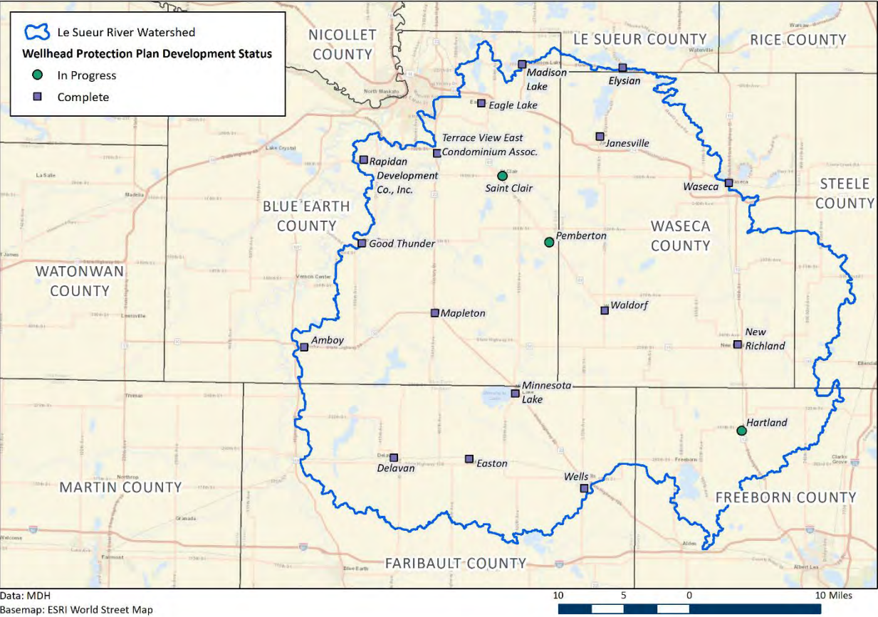
Figure 9: Le Sueur River Watershed - Wellhead Protection Plan Development Status for Community Public Water Systems. All except two of the 19 community public water supply systems are engaged in the wellhead protection planning process or are implementing their plans.
